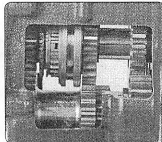
Model A Transmission with Mitchell Modification
