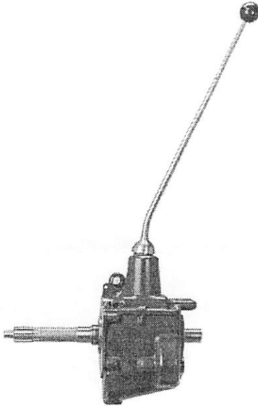
Standard Model A Transmission
